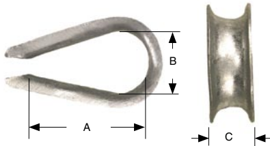
Standard Wire Rope Thimbles
