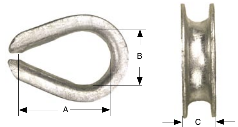
Heavy Duty Wire Rope Thimbles
